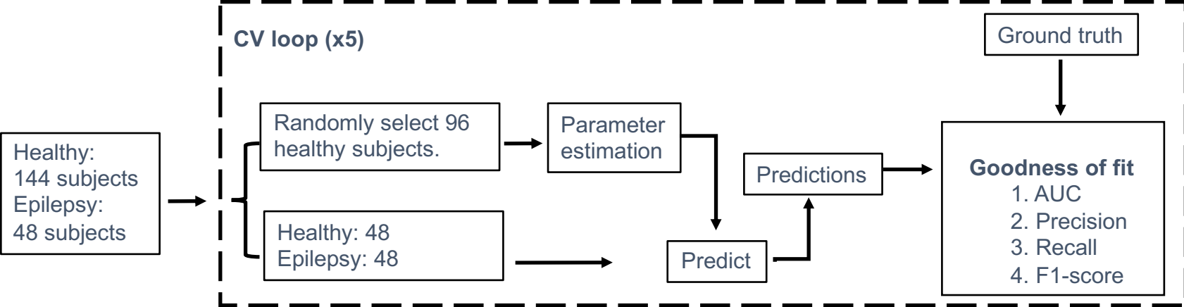
Figure 1: Classification framework. The mean of the alpha power distribution obtained from the data of 96 randomly chosen participants was calculated, separately for each channel. Then the deviations from this mean value for the rest of the participants were used to classify them as healthy or epilepsy, and the epilepsy patients were further classified for the epileptic side of brain. The predictions were compared against ground truth to evaluate the classification performance.
