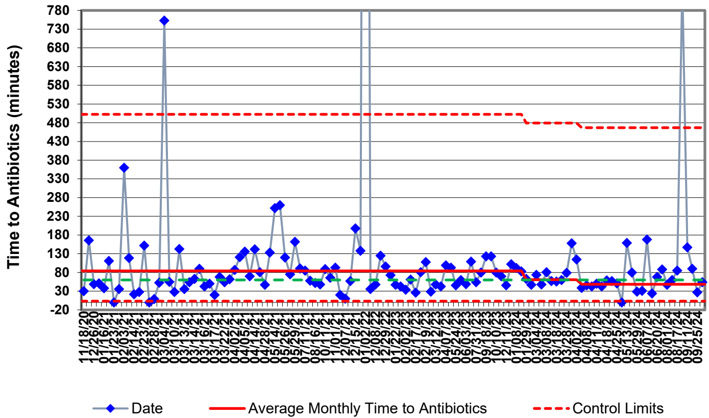
Time to Antibiotics X-Chart
