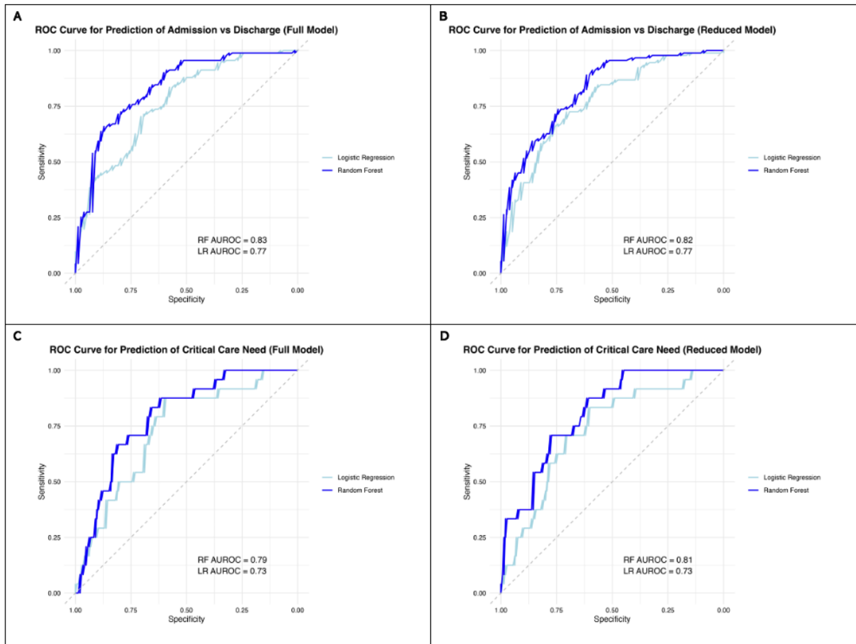
Figure 2: A) Receiver operator curve for the random forest and logistic regression classification models to predict hospital admission with all variables included (Full model). B) Receiver operator curve for the random forest and logistic regression classification models to predict hospital admission with select variables (Reduced model). C) Receiver operator curve for the random forest and logistic regression classification model to predict critical care need with all variables included (Full model). D) Receiver operator curve for the random forest and logistic regression classifier to predict critical care need with select variables (Reduced model). Note: ROC = receiver operator curve, AUROC = area under the receiver operator curve
