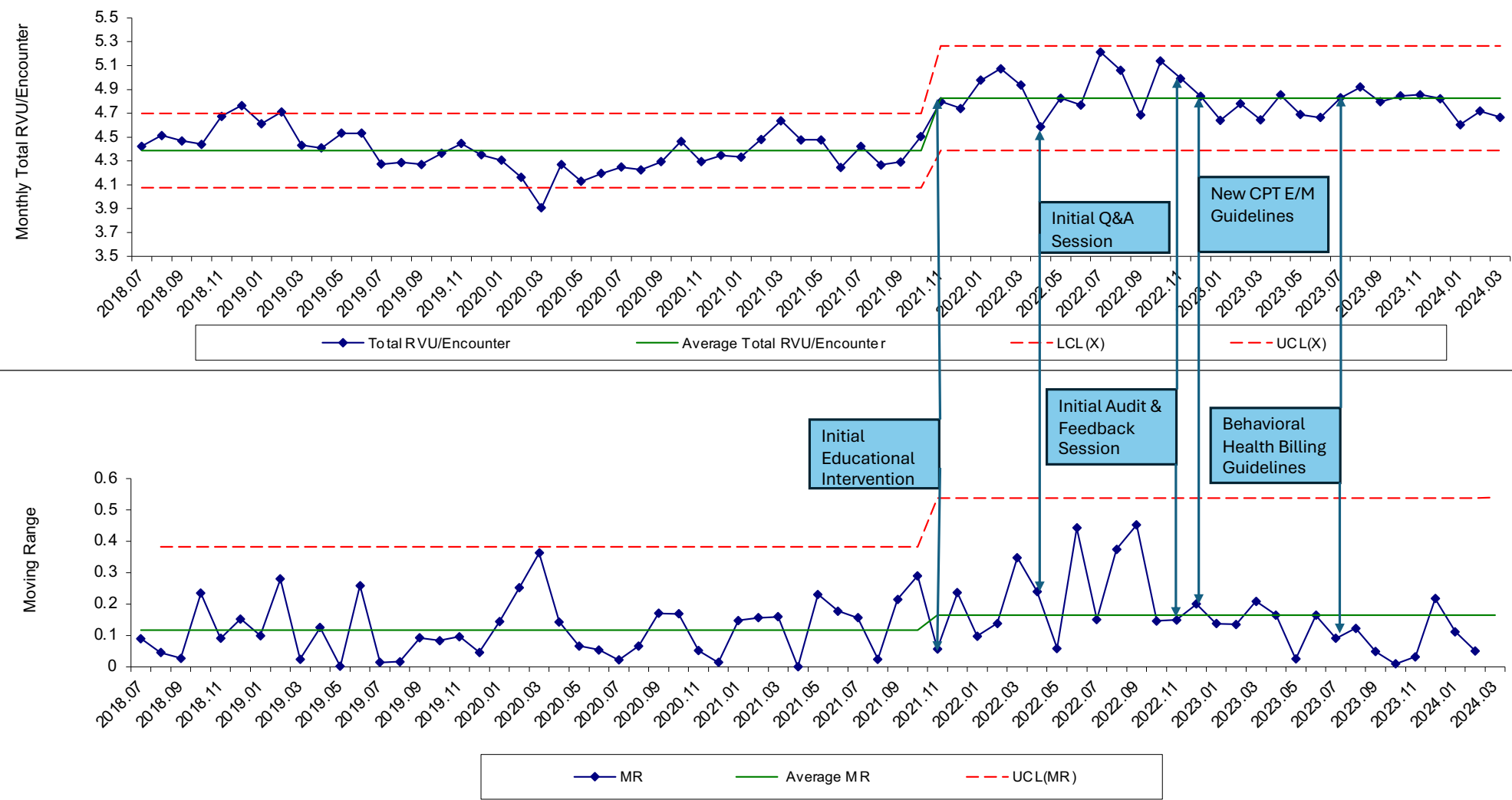
Figure 3. Monthly Total RVU/Encounter XmR Control Chart
