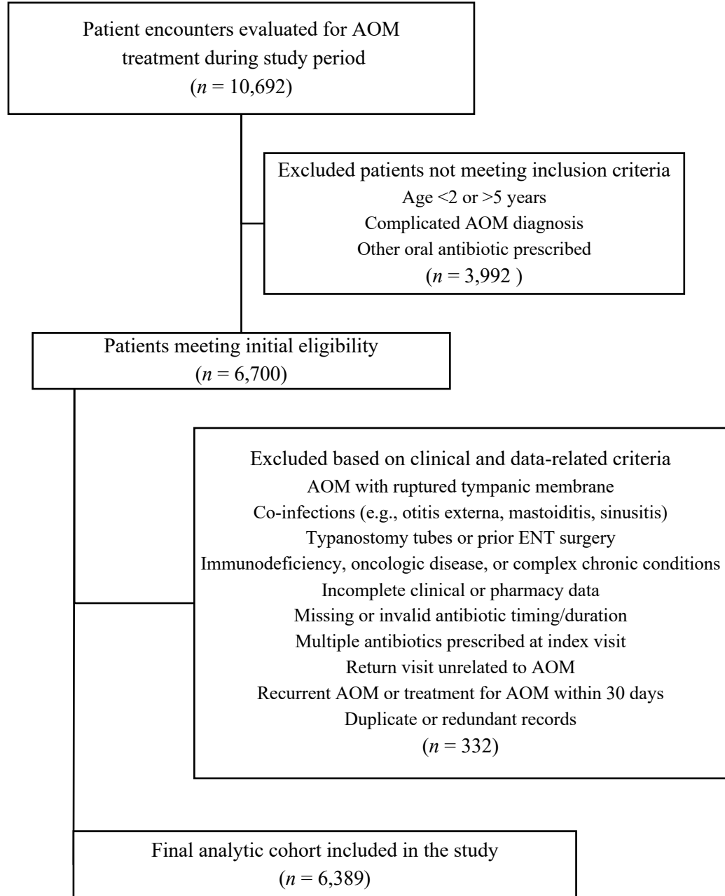
Figure 1. Overview of patient selection, inclusion, and exclusion. AOM=acute otitis media, ICD-10=international classification of diseases, ENT=ear, nose, and throat
