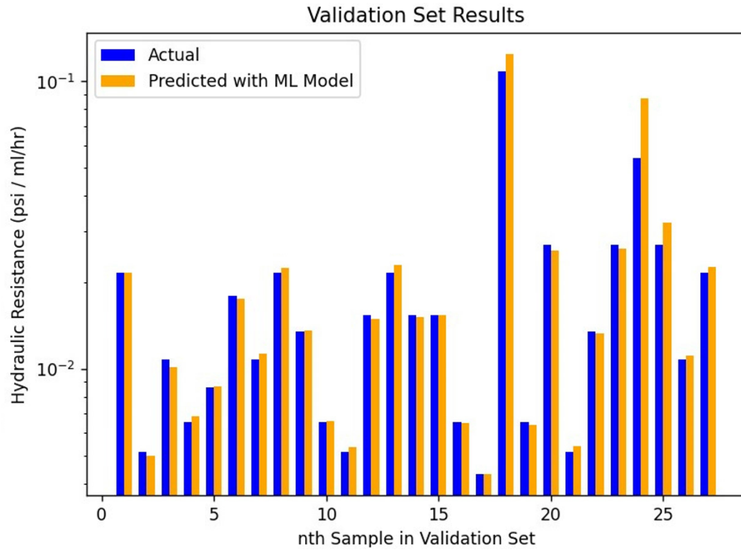
Figure 2. Actual vs. predicted obstruction with ML model, MSE = 5.32 \times 10^{-5} psi / ml/hr
